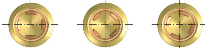
PRECIP-DIP contact with Eagle Grip - 4 fingers - size 16
