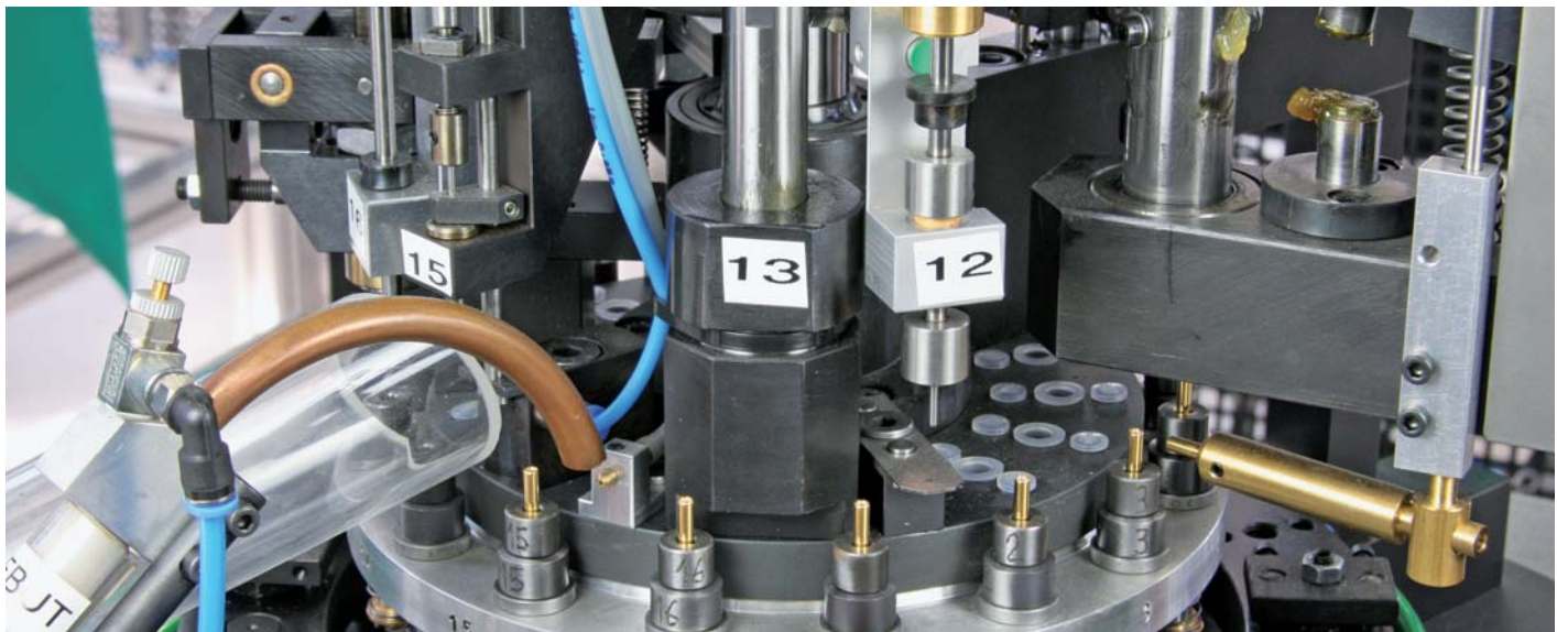
In-line mechanical and electrical checks are carried out on the assembly machine
